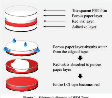
Figure 1. Schematic diagram of WDI Tape.
